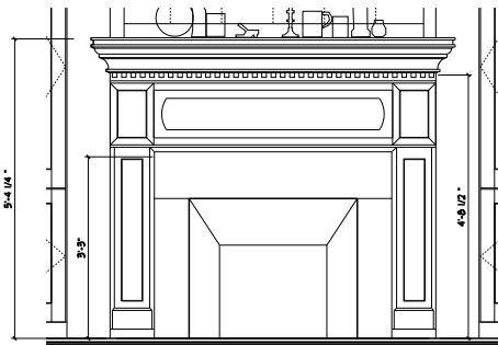
5 ELEVATION DETAIL FIREPLACE SCALE: 1" = 1'-0"
