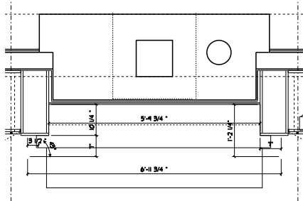
7 PLAN DETAIL FIREPLACE SCALE: 1" = 1'-0"
