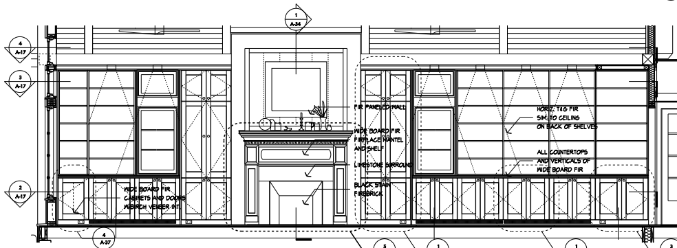
1 GREAT ROOM CABINET ELEVATION SCALE: 1/2" = 1'-0"
