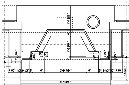
6 PLAN DETAIL FIREPLACE SCALE: 1" = 1'-0"
